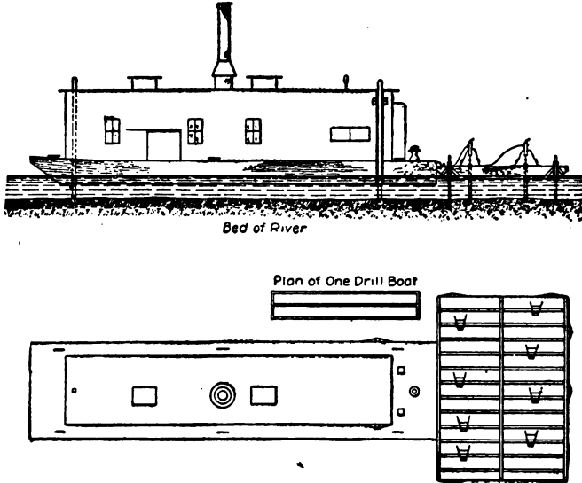
Fig. 173. Plan and Elevation of Drill Float and Tender, Tuscumbar Bar, Tennessee River.
